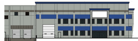
ENLARGED PARTIAL WEST ELEVATION 1/16" = 1'-0"
